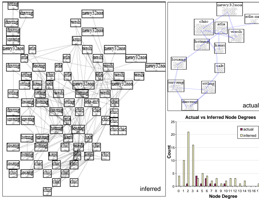
Figure 8: The IP alias resolution problem in practice. Shown is a comparison between the Abilene/Internet2 topology inferred by Rocketfuel (left) and the actual topology (top right). Rectangles represent routers with interior ovals denoting interfaces. The histograms of the corresponding node degrees are shown in the bottom right plot. (Reprinted from [141]; ©2008 ACM, Inc. Included here by permission.)
