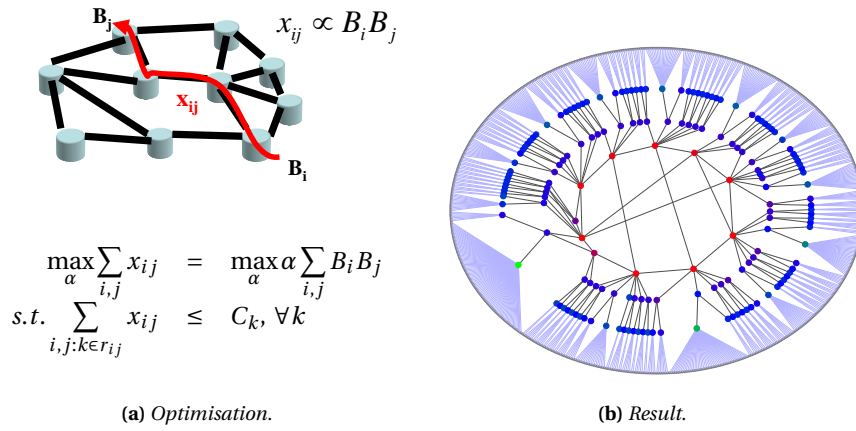
Figure 10: Generating networks using constrained optimization. (a) Engineers view network structure as the solution to a design problem that measures performance in terms of the ability to satisfy traffic demand while adhering to node and arc capacity constraints. (b) A network resulting from heuristically optimized tradeoffs (HOT). This network has very different structural and behavioral properties, even when it has the same number of nodes, links, and degree distribution as a scale free network shown in Figure 9. (First published in Notices of the American Mathematical Society , Volume 56, No.3 (May 2009): 586-599 [156]. Included here by permission.)
